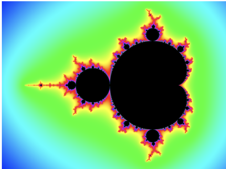
Figure 1: A high-resolution rendering of the classical Mandelbrot set ( j = 2 ), highlighting its aesthetic beauty. (Source: Geek3 via Wikimedia Commons [11], licensed under CC BY-3.0.)
