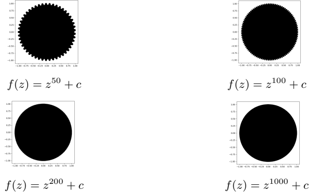
Figure 3: Representative Multibrot sets for f(z) = z^j + c . As the degree increases, the sets become increasingly circular and their boundaries progressively smoother. Images were generated using Python’s NumPy and Matplotlib libraries on a 1000 \times 1000 grid with an escape-time algorithm using 200 iterations.
